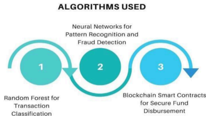
Fig 4: Algorithms Used
